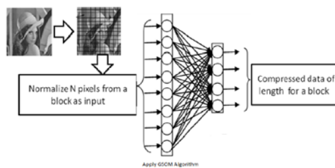
Figure 1: GSOM Architecture compression
