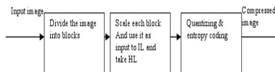
Figure 3: Encoding process of image compression
