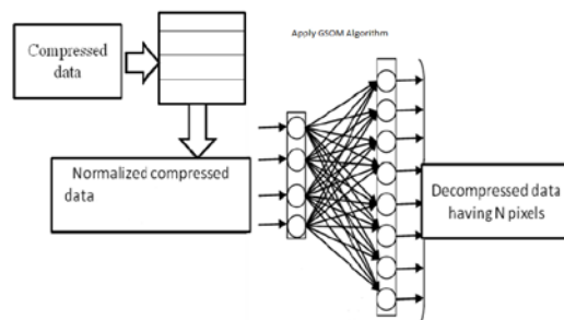
Figure 2: GSOM Architecture decompression
